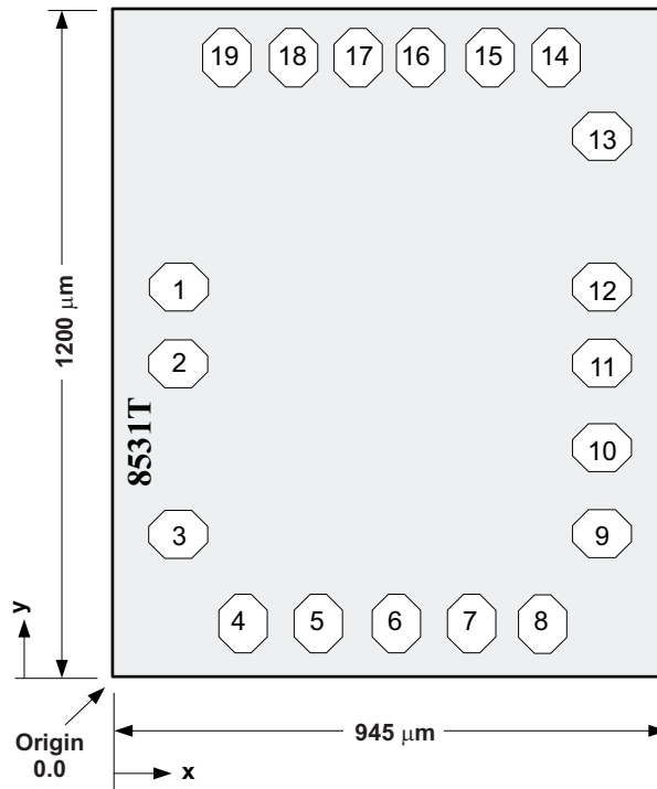
Bond Pad Locations and Descriptions
